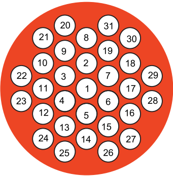
PLUG/FACE VIEW
