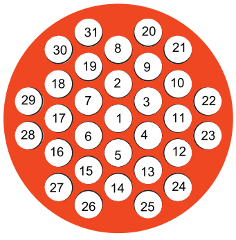
PIN/FACE VIEW
