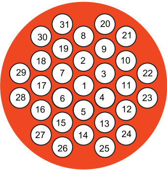
WIRE/REAR VIEW
